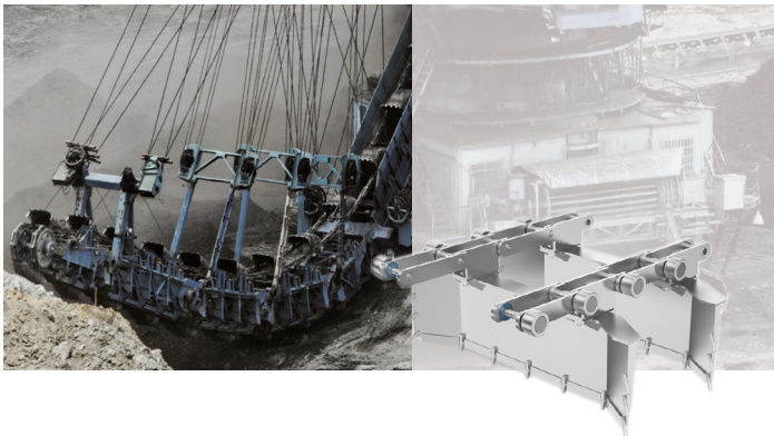
RECLAIMER CHAINS AND ROLLERS
